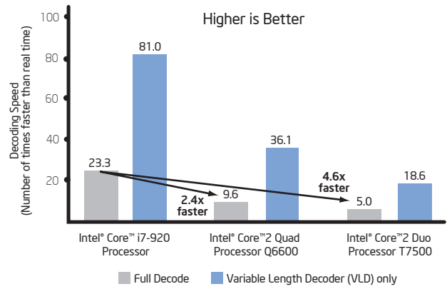
Figure 2. Decoding Speed 1
